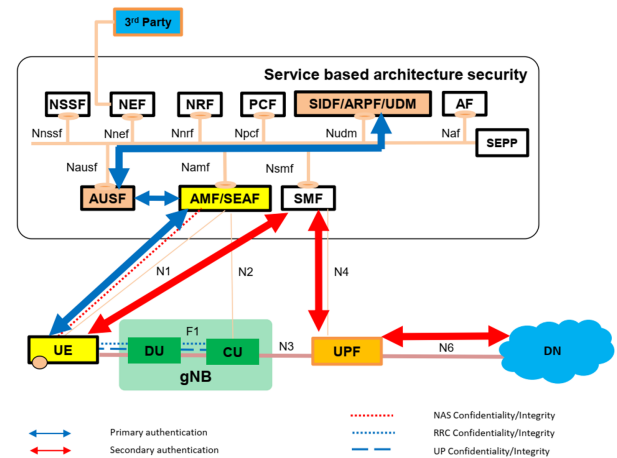
FIGURE 2: 5G Security Functions (extracted from [32])
