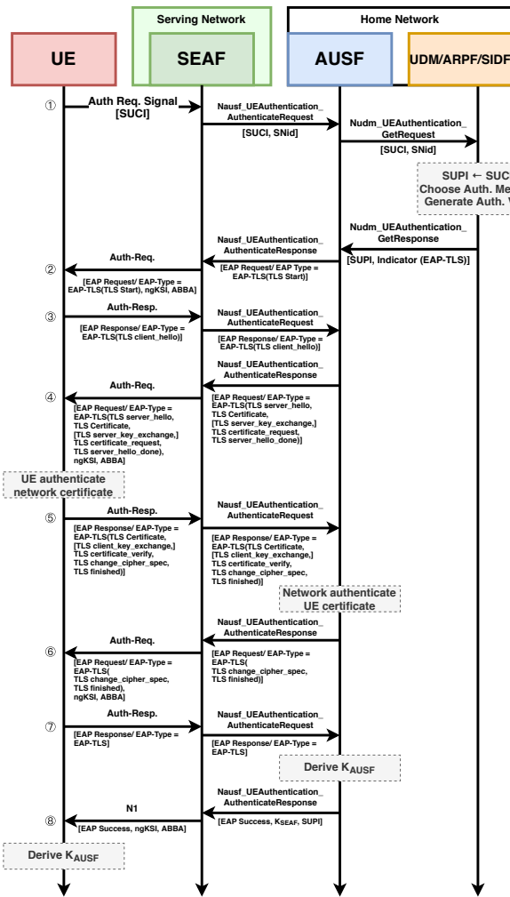
FIGURE 5: EAP-TLS authentication procedure over 5G networks for initial authentication
